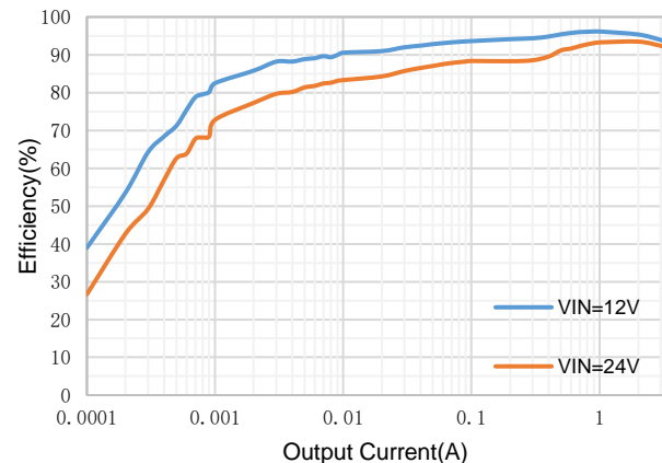
Efficiency, V_{OUT}=5V , F_{SW}=400KHz
