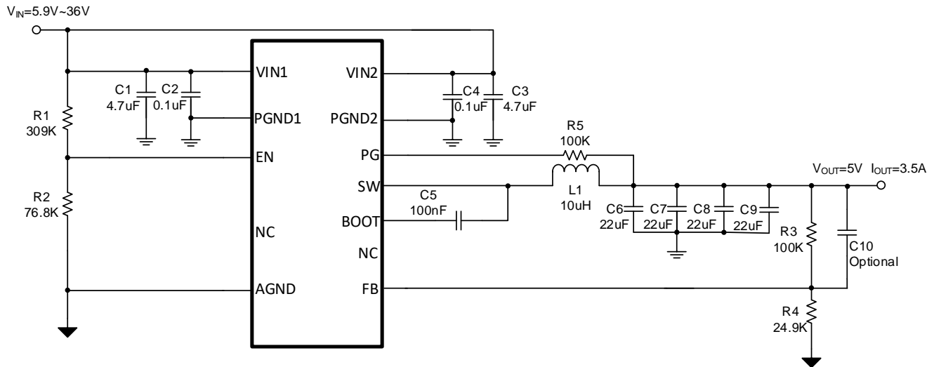
Figure 11. SCT2434AQ Design Example, 5V Output with Adjustable UVLO
