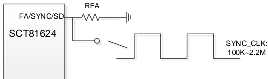
Figure16. Frequency Sync
