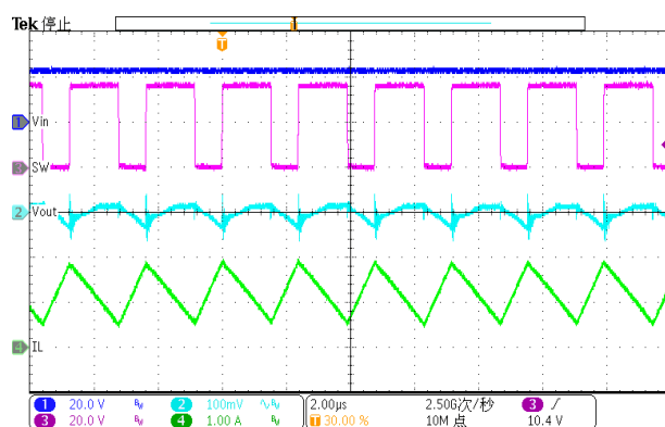
Figure 34. steady-state (Iload=2A)
