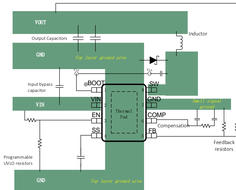
Figure 23. PCB Layout Example
