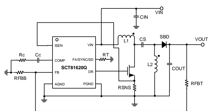
SEPIC
