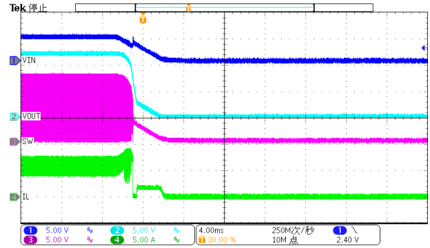
Figure 21. Power down(Iload=2A)
