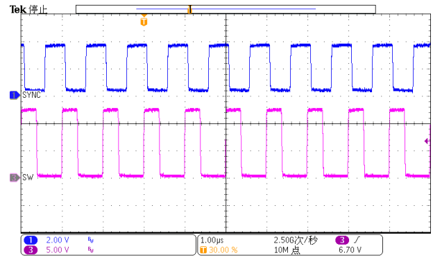
Figure 25. Sync Frequency
