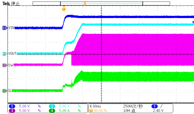
Figure 20. Power up(Iload=2A)
