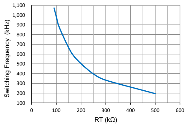
Figure 7. Clock Frequency vs RT/CLK Resistor
