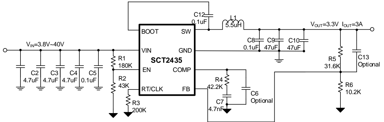
Figure 12. SCT2435 Design Example, 3.3V Output with Programmable UVLO
