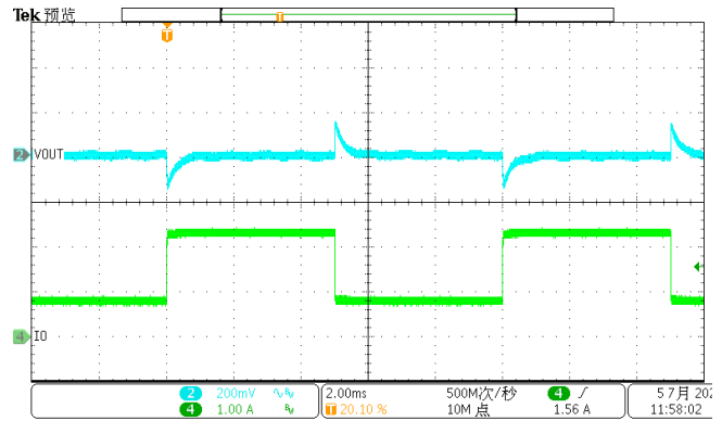
Figure 21. Load Transient (0.75A-2.25A, 1.6A/us)
