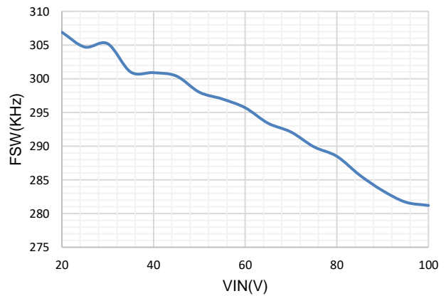
Figure 5. Switching Frequency VS Vin, Vout=12V
