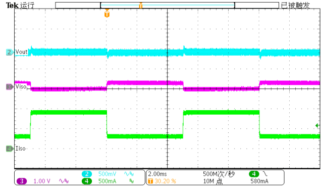
Figure 28. Load Transient 0.3A to 0.9A (isoload)
